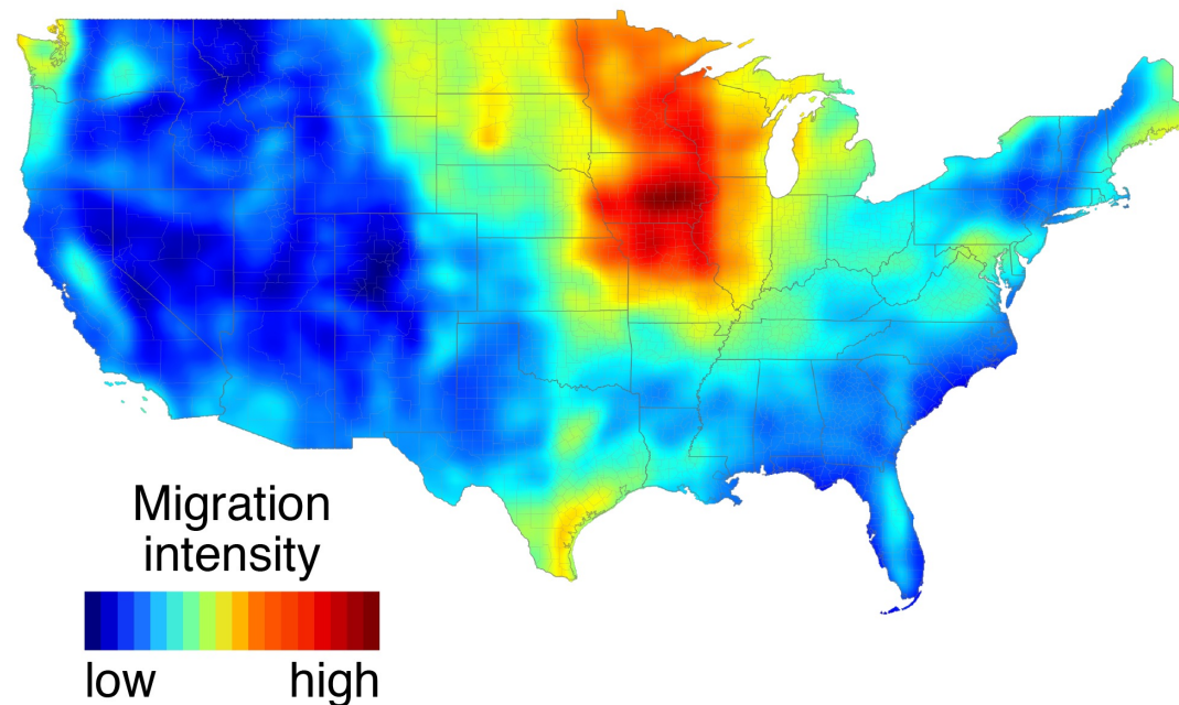
Bird migration forecast
